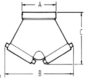
6405 Back Outlet
