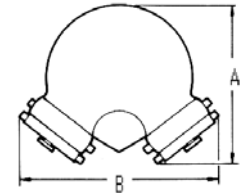
6405 Back Outlet
