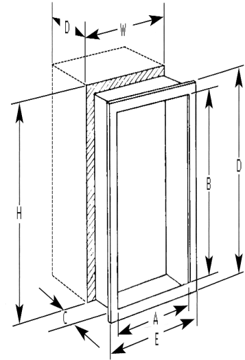
Tub for 1900 Series
